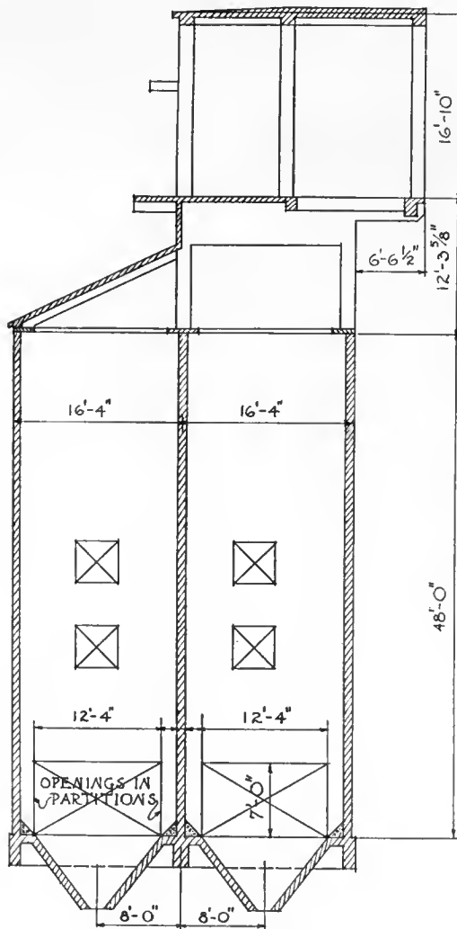
SECTION J-J LONGITUDINAL SECTION
